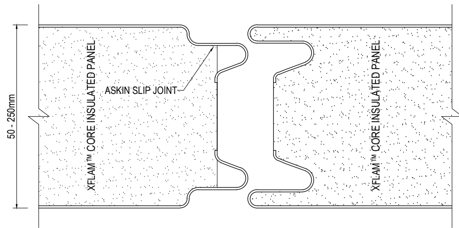
PANEL TO PANEL CONNECTION DETAIL SCALE 1:1
